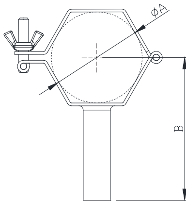
Wing Nut
