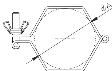
Wing Nut
