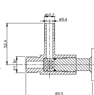
SAMPLING VALVE PIPE THREAD-1/2"
