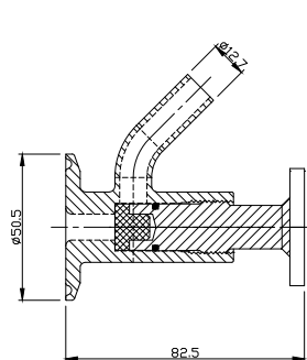
SAMPLING VALVE 45°CLAMP END-1.5"
