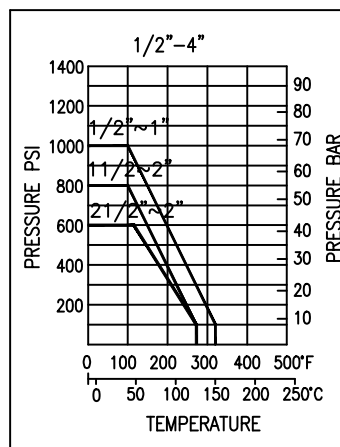
PRESSURE TEMPERATURE RATING
