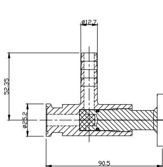
SAMPLING VALVE CLAMP END-3/4"
